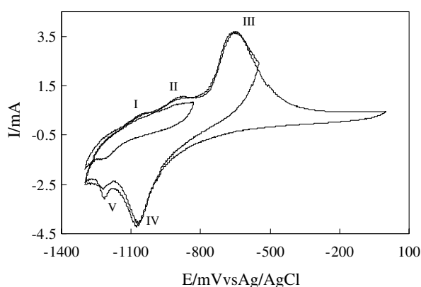
Fig. 3. Effect of different potential limits on cyclic voltammograms in pure NaOH solution at 30 \text{ }^\circ\text{C} , dE/dt = 50 \text{ mV s}^{-1} .
