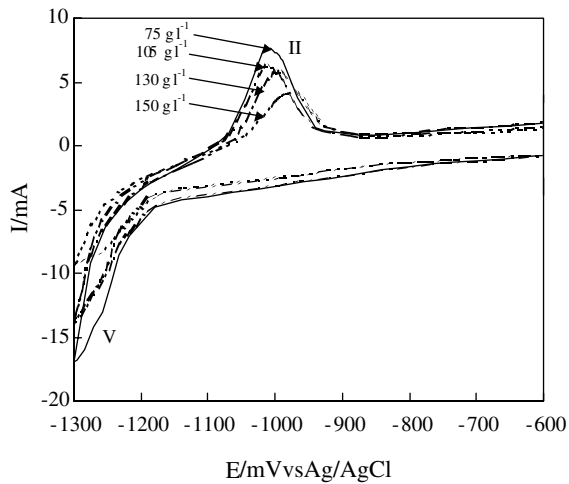
Fig. 5. Influence of alumina content on stable voltammogram, dE/dt = 50 \text{ mV s}^{-1} . Key: (—) 75 , (---) 105 , (···) 130 and (-·-) 150 \text{ g l}^{-1} .
