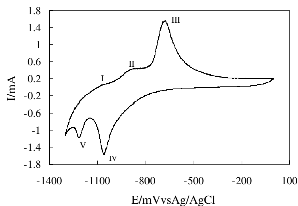
Fig. 1. Stable voltammogram of 300W in 2.25 M NaOH solution at 30 \text{ }^\circ\text{C} , dE/dt = 50 \text{ mV s}^{-1} .
