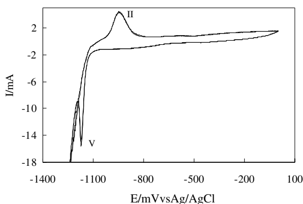
Fig. 2. Stable voltammogram of 300W in 2.25 M NaOH solution at 100 \text{ }^\circ\text{C} , dE/dt = 50 \text{ mV s}^{-1} .
