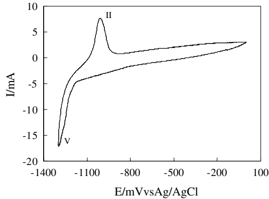
Fig. 4. Stable voltammogram of 300W obtained in a Bayer solution with 75 \text{ g l}^{-1} of alumina at 100 \text{ }^\circ\text{C} , dE/dt = 50 \text{ mV s}^{-1} .
