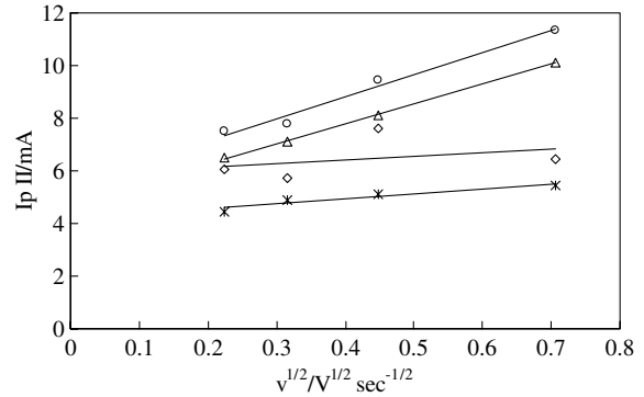
Fig. 6. Variation of peak II current for different alumina concentrations and scan rates. Key: (○) 75 , (△) 105 , (◇) 130 and (*) 150 \text{ g l}^{-1} .
