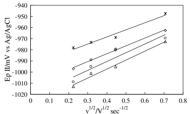
Fig. 7. Variation of peak II potential for different alumina concentrations and scan rates. Key: (○) 75 , (△) 105 , (◇) 130 and (*) 150 \text{ g l}^{-1} .
